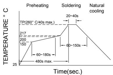
Figure 1. Re-flow Soldering
