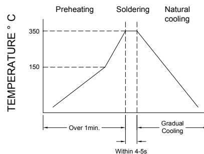
Figure 2. Iron Soldering
